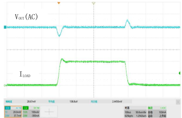
图 21. 负载瞬态响应, V_{IN}=4.3V , V_{OUT}=3.3V , I_{OUT}=1mA to 150mA
