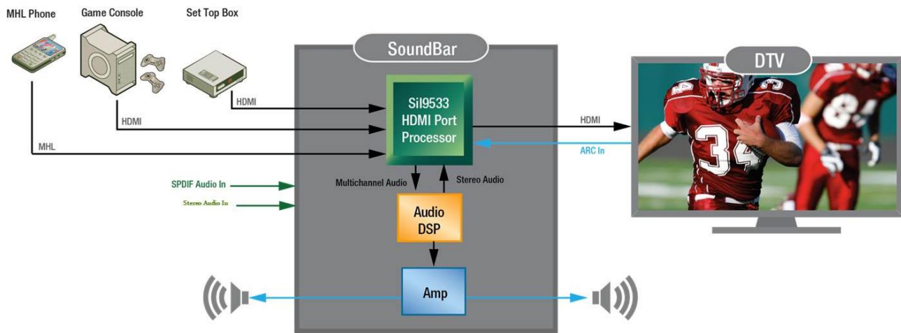
Figure 1.2. Typical SoundBar Application
