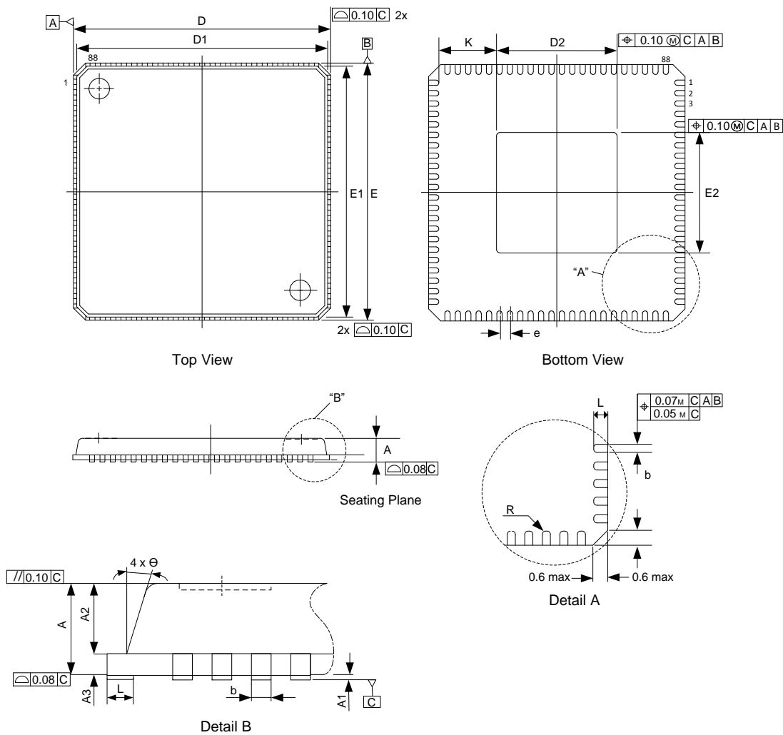
Figure 8.1. Package Diagram
