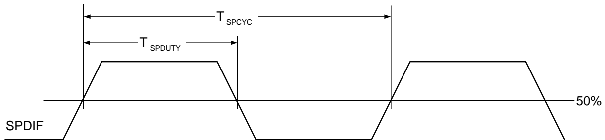
Figure 4.7. S/PDIF Output Timing
