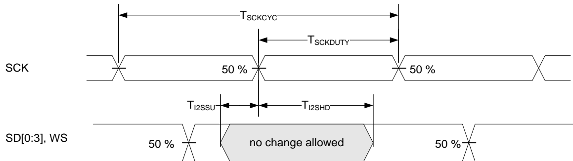
Figure 4.4. I 2 S Input Timing
