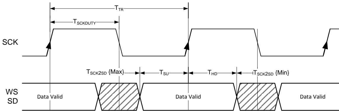
Figure 4.6. I 2 S Output Timing
