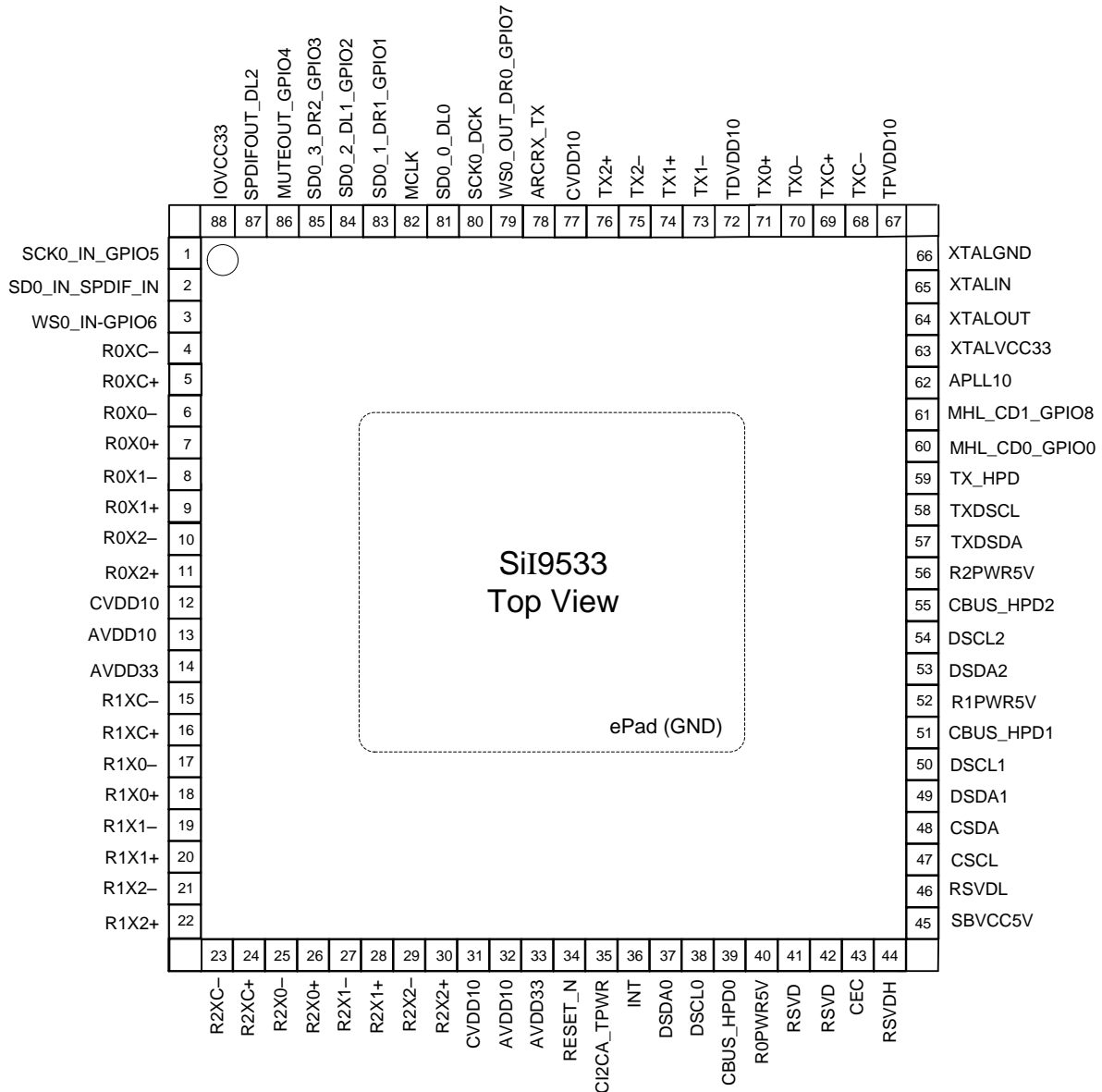
Figure 5.1. Pin Diagram
