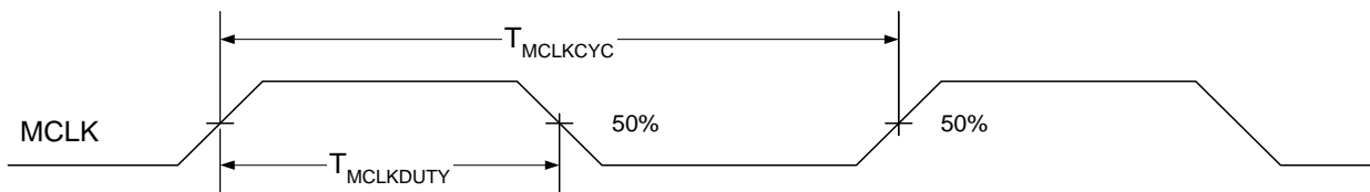
Figure 4.8. MCLK Timing
