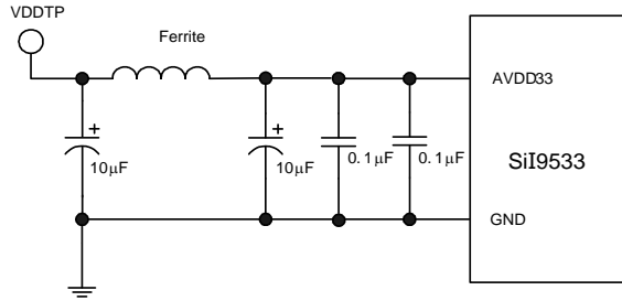
Figure 3.1. Test Point VDDTP for AVDD33 Noise Tolerance Specification
