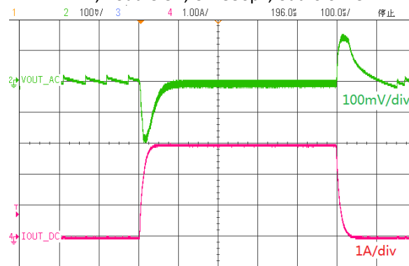
Load Transient
