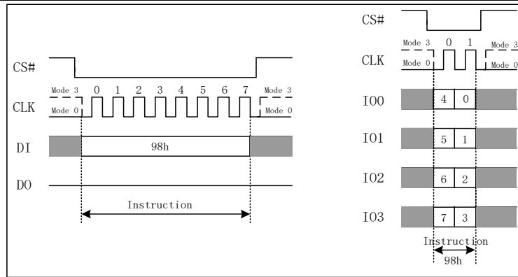
Figure 7.40 Global Block Lock Instruction (SPI or QPI Mode)
