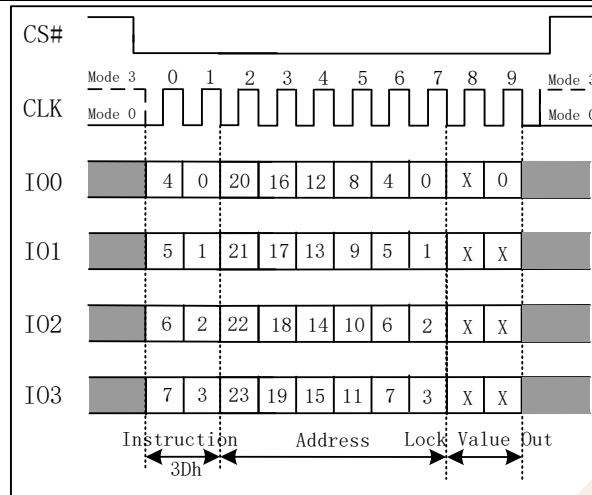
Figure 7.38b Read Block Lock Instruction(QPI Mode)
