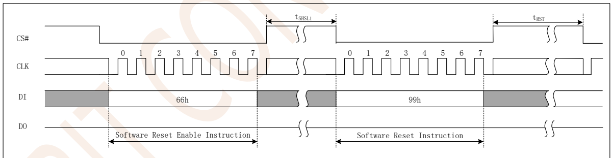
Figure 8.7 Reset Input Timing
