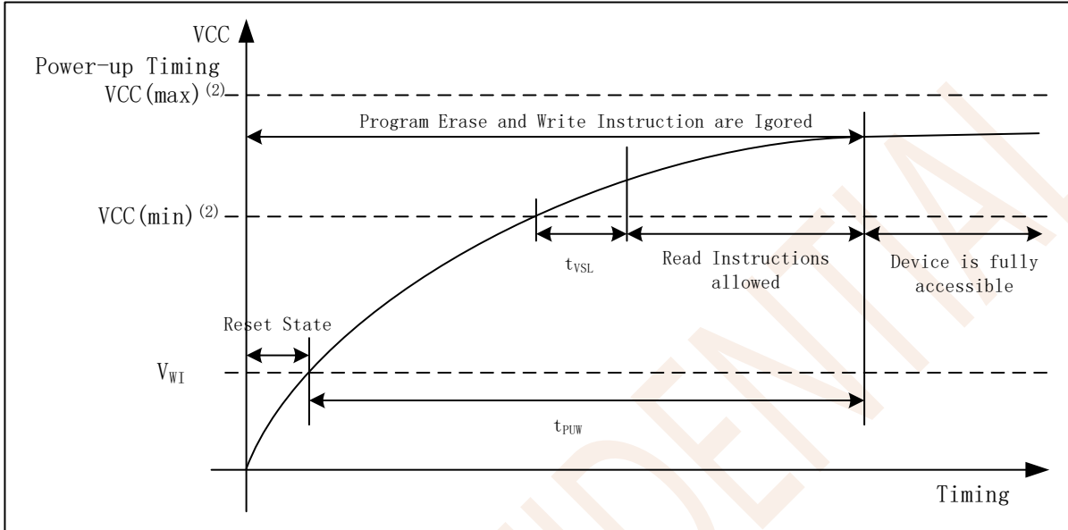
Figure 8.1 Power-up Timing
