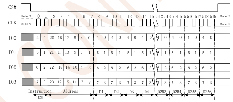
Figure 7.6b Page Program Instruction (QPI Mode)
