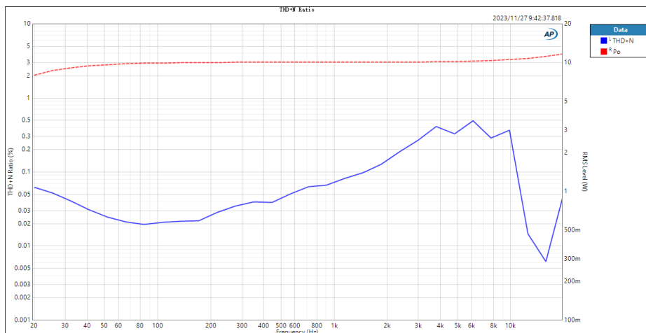
frequency vs THD+N ( P_o \approx 10\text{W} )
