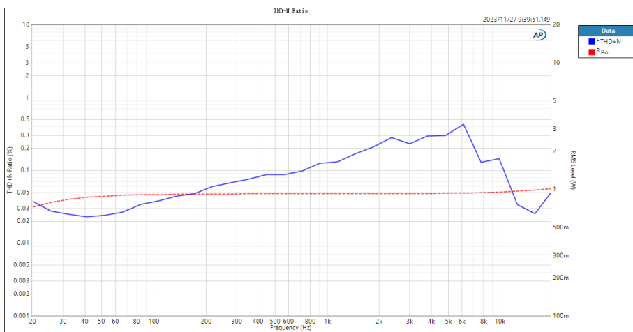
frequency vs THD+N ( P_o \approx 1\text{W} )
