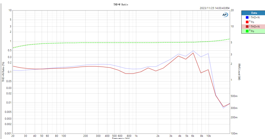
frequency vs THD+N ( P_o \approx 2 \times 5\text{W} )
