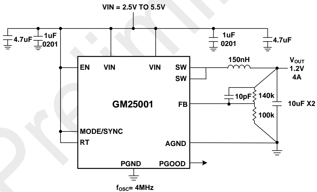
图 8. 4MHz, V IN =3.3V, V OUT =1.2V, I LOAD =4A
