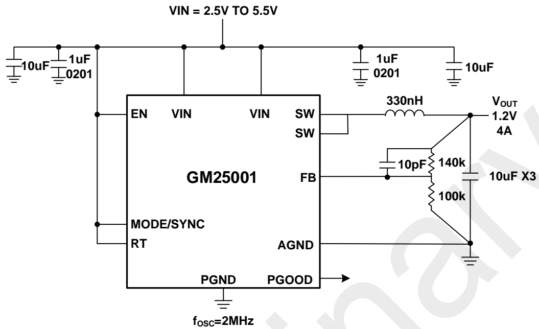
图 7. 2MHz, V IN =3.3V, V OUT =1.2V, I LOAD =4A
