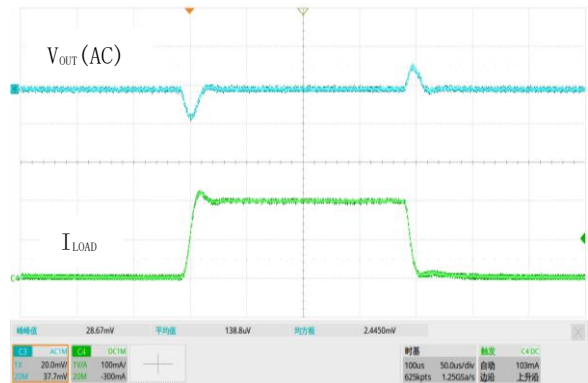
图 22. 负载瞬态响应, V_{IN}=4.3V , V_{OUT}=3.3V , I_{OUT}=1mA to 200mA
